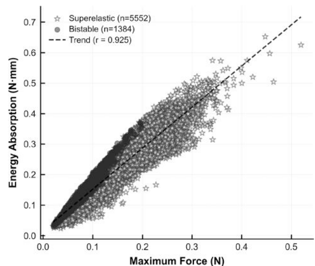
Fig. 2 Dataset overview: peak force and energy absorption across 6936 classified unit cell designs. Each point represents a single unit cell design plotted by its peak force (horizontal axis) and energy absorbed per loading–unloading cycle (vertical axis). Superelastic designs (stars, n = 5552 ) occupy the upper portion; bistable designs (circles, n = 1384 ) cluster toward the lower end. A trend line ( r = 0.925 ) shows that the two quantities are coupled across the dataset, reflecting the shared geometric origin of both properties.
