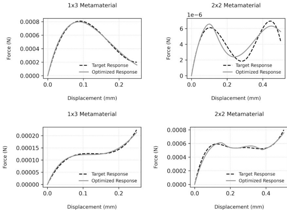
Fig. 5 Surrogate optimization results for single-surface loading. Each panel compares the desired force–displacement curve (dashed) with the surrogate force at the optimized polynomial coefficients (solid). Results are shown for a 1 \times 3 configuration (left) and a 2 \times 2 configuration (right), each for two different desired shapes. For the single-row configuration, agreement is close across the full displacement range.
