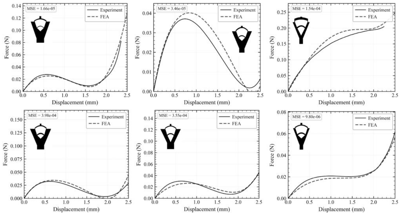
Fig. 10 Measured force–displacement curves compared with finite element predictions for six fabricated designs. In each panel, the solid curve is the experimental measurement and the dashed curve is the finite element prediction obtained from the shape parameters returned by the machine learning model; the MSE between the two is reported in each panel inset. The unit cell geometry is shown alongside each panel. The six designs span the full behavioral range intended by the process: superelastic responses at different peak forces, constant-force response, and bistable responses with different levels of energy absorption.
