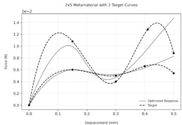
Fig. 7 Multi-surface optimization result for a 2 \times 5 metamaterial. The optimized force–displacement response (solid) is shown alongside both desired curves (dashed). The surrogate identifies polynomial coefficients for each unit cell such that the response at both loading surfaces matches its respective target. The two curves are qualitatively distinct, confirming that the multi-surface formulation can encode different mechanical behaviors in different regions of a single continuous material.
