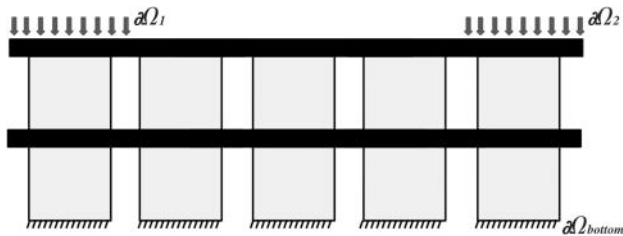
Fig. 6 Multi-surface loading configuration. A 2 \times 5 metamaterial with two distinct loading surfaces, \partial\Omega_1 (top left) and \partial\Omega_2 (top right), each subjected to an independent prescribed displacement. The bottom surface is fixed. Each surface can be assigned a different desired force–displacement curve, so that distinct mechanical behaviors are encoded in different regions of a single continuous structure.
