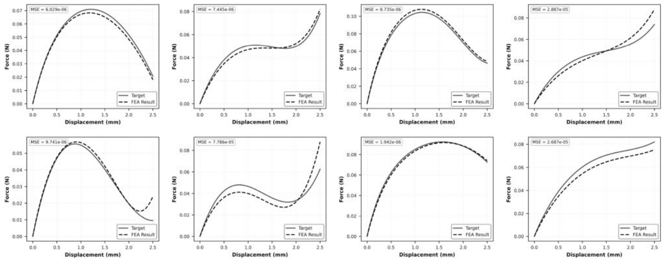
Fig. 8 Machine learning predictions verified by finite element simulation. Each panel shows an intended force–displacement curve (solid) and the curve produced by simulating the geometry predicted by the network (dashed, labeled FEA result). Eight representative examples are shown, covering the range of curve shapes in the dataset. The MSE between target and finite element result is reported in each panel. Agreement is close for most examples; the largest deviations occur near sharp peaks, where the geometry-to-response mapping is most sensitive to small changes in shape parameters.
