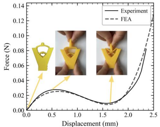
Fig. 9 Force–displacement response and deformation stages of a representative unit cell. The experimental measurement (solid line) shows agreement with the finite element prediction (dashed line). Inset photographs illustrate the physical deformation at key points along the response curve: the initial undeformed state (left), the onset of snap-through instability near the local peak force (middle), and the highly deformed buckled configuration at the local force minimum (right).
