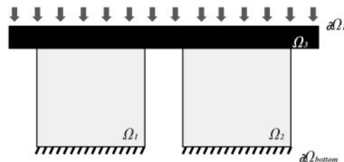
Fig. 4 Surrogate model of a 2 \times 1 metamaterial. The two physical unit cells are replaced by rectangular domains \Omega_1 and \Omega_2 , each governed by a polynomial energy density. A Neo-Hookean layer \Omega_3 connects both domains to the prescribed displacement boundary \partial\Omega_1 (top, arrows). The fixed bottom boundary \partial\Omega_{\text{bottom}} is indicated by hatching.
