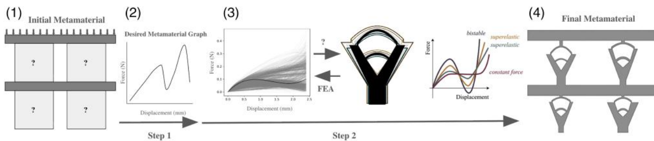
Fig. 3 The inverse design pipeline: (1) a surrogate model, in which each unit cell is replaced by a polynomial energy density, is optimized to match the target, yielding the required force–displacement behavior of each unit cell; (2) a desired force–displacement curve is specified for the assembled metamaterial; (3) a machine learning model maps each required unit cell response to the 11 shape parameters that produce it, using the finite element dataset; and (4) the resulting example unit cell geometries are assembled into the full metamaterial. Arrows show the direction of information flow.
