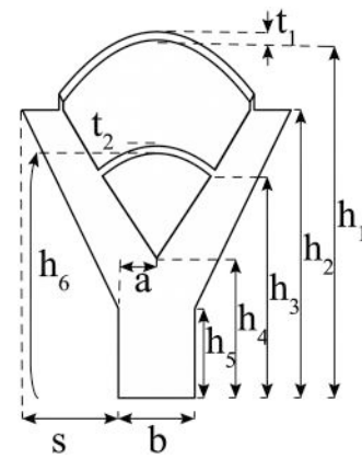
Fig. 1 Unit cell topology and shape parameters. The unit cell is defined by 11 parameters: heights h_1 – h_6 , widths t_1 , t_2 , s , and b , and curvature offset a . These parameters control the geometry of the upper and lower curves. Varying them within the fixed topology produces the full range of superelastic and bistable responses observed in the dataset.
